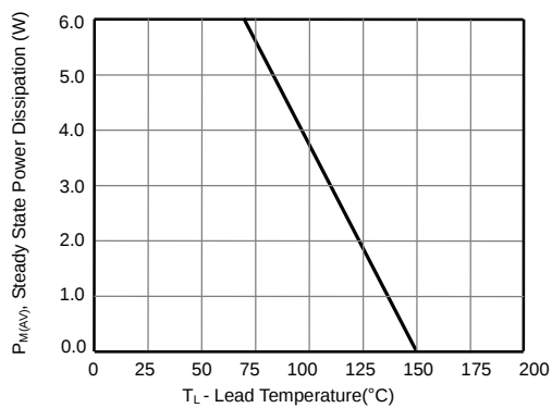
Figure 5-SteadyStatePower Derating Curve
