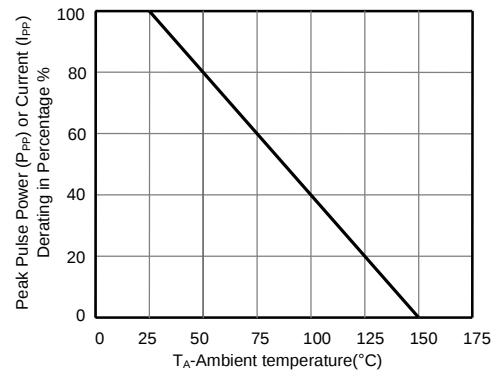
Figure 2 -Pulse DeratingCurve
