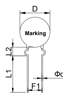
O Type (外弯脚)
