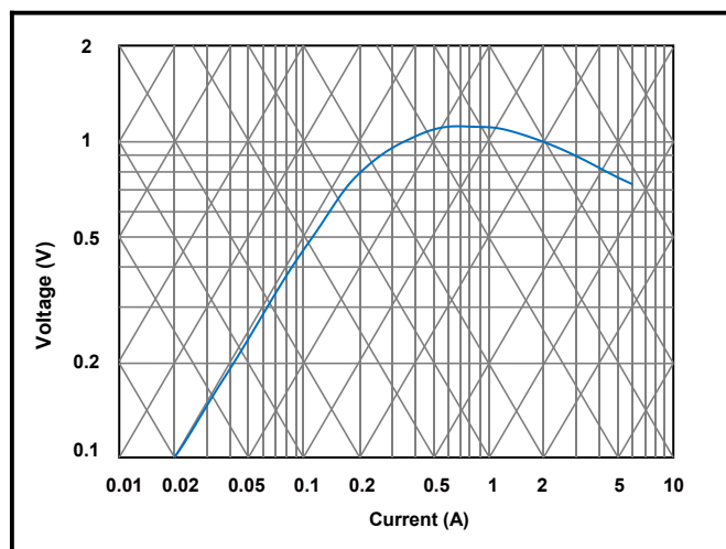
Figure 2 - Graph of Voltage vs. Current
